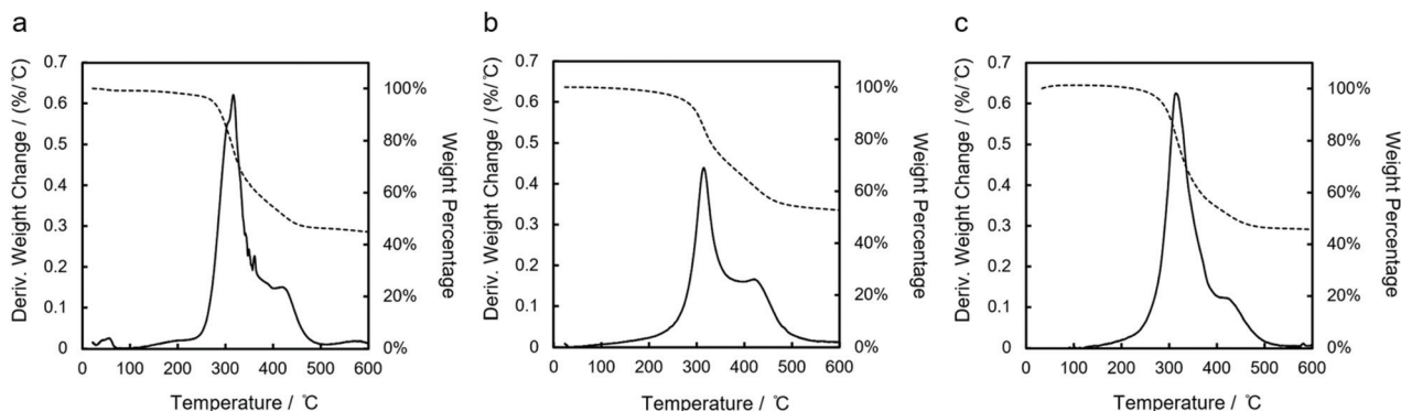
Fig. 5 TGA curves of (a) lin -poly( 1,4Si 6 ), (b) cyc -poly( 1,3Si 6 ) and (c) lin -poly( 1,3Si 6 ). Solid lines: derivative weight change; dotted lines: percentage weight change.
