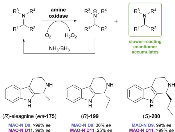
Scheme 24 General reaction scheme for the 'cyclic deracemisation' of amines, and examples of tetrahydro-β-carbolines that have been deracemised using engineered variants of MAO-N.
