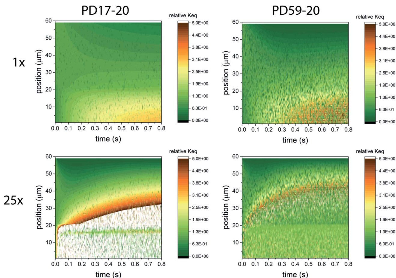
Fig. 4 Maps of the ratio ([I_3^-]/[I^-][I_2])/K_{eq} as a function of position and time in the electrolyte, as a measure of deviation from expected equilibrium concentrations under Sc2. The photoanode contact is at 0 \mu\text{m} , the interface between the photoanode and bulk electrolyte is at 20 \mu\text{m} , and the cathode is at 60 \mu\text{m} . In the simulations 1 particle represents 3 \times 10^{14} \text{ mol cm}^{-3} . Whenever the ion concentration is 0 particles, it is set to a value of 6 \times 10^{13} \text{ mol cm}^{-3} to permit these ratios to be calculated. (a) 1 \text{ s}^{-1} excitation frequency, PD17-20, (b) 25 \text{ s}^{-1} excitation frequency, PD17-20, (c) 1 \text{ s}^{-1} excitation frequency, PD59-20, (d) 25 \text{ s}^{-1} excitation frequency, PD59-20. Data for Sc1 are nearly indistinguishable from this set.
