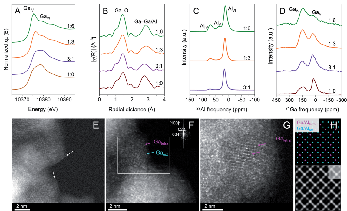
Fig. 2 Structural characterization of the calcined (\text{Ga,Al})_2\text{O}_{3(x:y)} materials. (A) Ga K-edge XANES spectra, and (B) Fourier transform of the EXAFS data of (\text{Ga,Al})_2\text{O}_{3(x:y)} NPs. Captions in (A) indicate features corresponding to \text{Ga}_{\text{IV}} and \text{Ga}_{\text{VI}} sites and captions of the peaks in (B) indicate the Ga–O and Ga–Ga/Al coordination sphere. Panels (C) and (D) show ^{27}\text{Al} and ^{71}\text{Ga} MAS NMR spectra, respectively, obtained at 700 MHz in 1.3 mm rotors spun at 50 kHz. (E) ADF-STEM images of (\text{Ga,Al})_2\text{O}_{3(1:3)} showing terminating rows of octahedral cation sites. In (F), the region in the white box features a spinel-type structure oriented along the [100]-zone axis (FFT pattern is shown in the top right inset), with arrows indicating Ga atoms in tetrahedral and octahedral crystallographic positions. In (G), the image shows a (\text{Ga,Al})_2\text{O}_{3(1:6)} particle, also oriented along the [100]-zone axis, where the arrows indicate preferential occupation of tetrahedral sites by Ga. The spinel model in (H) shows Ga occupying both tetrahedral and octahedral positions, as in the case of (\text{Ga,Al})_2\text{O}_{3(1:3)} . (I) Shows an ADF-STEM model for the spinel structure along the [100]-zone axis, where Ga and Al occupy tetrahedral and octahedral positions, respectively.
