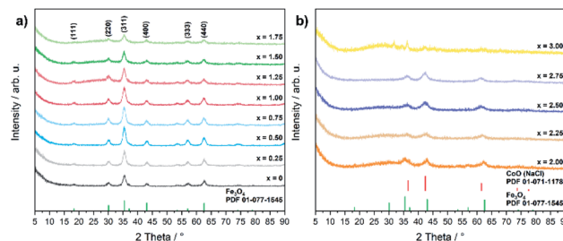
Fig. 1 PXRD patterns of (a) \text{Co}_x\text{Fe}_{3-x}\text{O}_4 ( x = 0–1.75 ) and (b) \text{Co}_x\text{Fe}_{3-x}\text{O}_4/(\text{Co}_x/3\text{Fe}_{1-x}/3)\text{O} ( x = 2–3 ) with references for \text{Fe}_3\text{O}_4 (PDF 01-077-1545) and \text{CoO} (PDF 01-071-1178).
