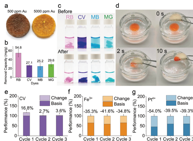
Fig. 4 Water purification performance. (a) Reduced Au 3+ into Au nanoparticles and metallic gold on top of the aerogel. (b and c) Dye removal performance. (d) Rapid removal of organic solvents from water. (e–g) Changes of adsorption performance after three regeneration cycles.
