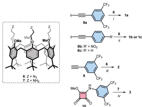
Scheme 1 Synthesis of receptors 1–3 from precursor calix[6]arenes 6 and 7 . Conditions: (i) \text{CuI} , TBTA, THF; (ii) [\text{Cu}(\text{CH}_3\text{CN})_6]\text{PF}_6 , TBTA, THF; (iii) [\text{Cu}(\text{CH}_3\text{CN})_6]\text{PF}_6 , 2,6-lutidine, DCM; (iv) DIPEA, MeOH, DCM.
