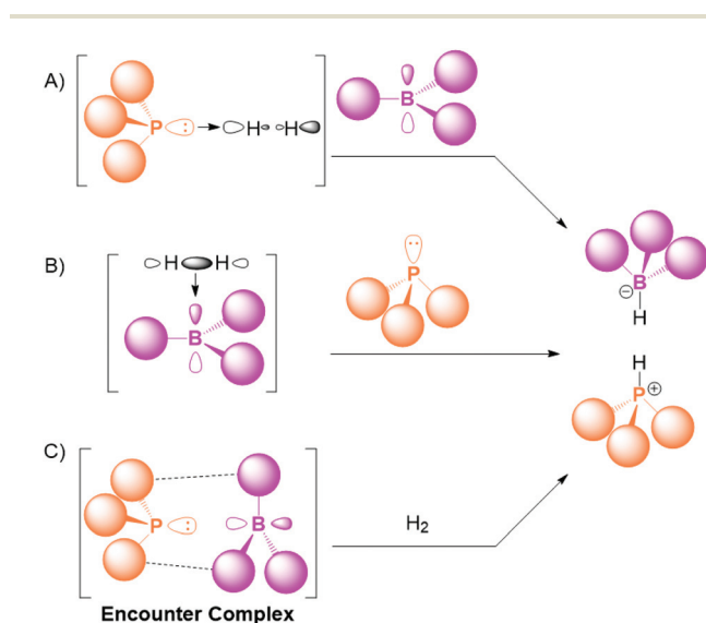
Scheme 1 Mechanisms for the splitting of H_2 by an FLP comprising a bulky phosphine and borane as alternatives to true termolecular reactivity. A: pre-association of the phosphine and H_2 ; B: pre-association of the borane and H_2 ; and C: pre-association of the phosphine and borane as an encounter complex.
