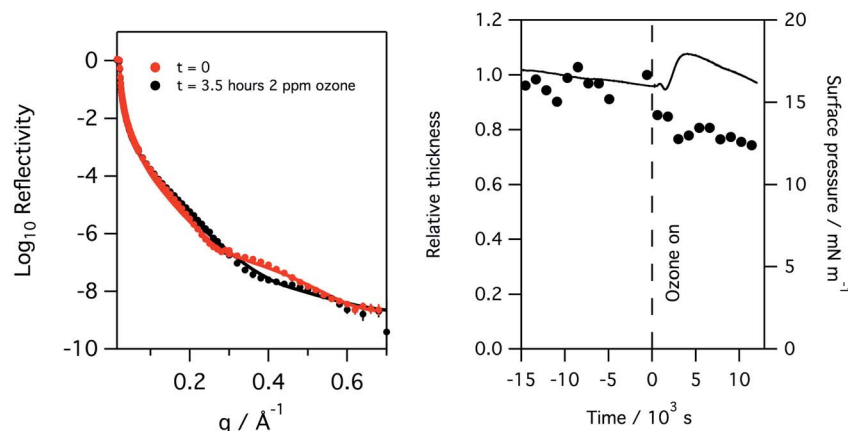
Fig. 6 Left: reflectivity of a monolayer of ovine lung surfactant at the air/water interface to X-rays at the start and after 3.5 hours of exposure to 2 ppm of ozone in oxygen gas. Right: plot of surface pressure (black line), fitted relative thickness (black circles) with time for the monolayer. As in the case of the porcine surfactant, a rapid drop in layer thickness is observed upon exposure to ozone.
