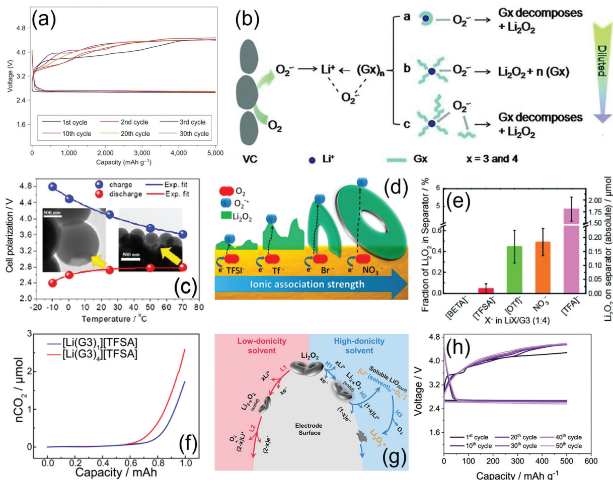
Fig. 8 (a) Voltage profiles of a \text{Li}[\text{G}_4\text{-LiTf}]\text{O}_2 battery under a 5000 \text{ mA h}^{-1} specific-capacity limit with reference to the mass of carbon cast on the cathode GDL; current rate: 500 \text{ mA g}^{-1} (current rate with reference to the mass of carbon cast on the cathode GDL). Adapted with permission. 144 Copyright © 2012 Macmillan Publishers Limited. All rights reserved. (b) Mechanism of the \text{O}_2 reduction reaction in a \text{Li-O}_2 cell at the interface between carbon black and glyme- \text{LiTFSI} electrolyte solution as proposed elsewhere. Reproduced with permission. 109 Copyright © 2013 WILEY-VCH Verlag GmbH & Co. KGaA, Weinheim. (c) Trends of charge (blue) and discharge (red) voltage vs. temperature for a \text{Li-O}_2 cell using a \text{G}_4\text{-LiTf} electrolyte solution. Insets: ex situ TEM images of the cathode of the same cell after galvanostatic discharge at 25^\circ\text{C} (left-hand side) and at 70^\circ\text{C} (right-hand side); capacity limited to 10\,000 \text{ mA h g}^{-1} with reference to the mass of carbon cast on the cathode GDL; current rate: 500 \text{ mA g}^{-1} (current rate with reference to the mass of carbon cast on the cathode GDL). Reproduced with permission. 111 Copyright © 2013 American Chemical Society. (d) Schematic representation of the effect of salt anions (i.e., \text{TFSI}^- , \text{Tf}^- , \text{Br}^- , and \text{NO}_3^- ) in electrolyte solutions based on \text{G}_2 on the kinetics and thermodynamics of the ORR, as well as on the morphology of electrodeposited \text{Li}_2\text{O}_2 in \text{Li-O}_2 batteries. Reproduced with permission. 117 Copyright © 2016 American Chemical Society. (e) Results of quantitative determination of \text{Li}_2\text{O}_2 on the separator in a \text{Li-O}_2 cell using \text{LiX/G}_3 (1:4) electrolytes, where \text{X}^- = \text{BETI}^- , \text{TFSI}^- , \text{Tf}^- , \text{NO}_3^- , and \text{TFA}^- . The values on the left y-axis are the percentage of the amount detected in the separator with respect to the amount of total expected (theoretical) \text{Li}_2\text{O}_2 present in the cell after discharge to 1 \text{ mA h cm}^{-2} , whilst the corresponding absolute values ( \mu\text{mol} ) are shown on the right y-axis; error bars denote the standard error. Adapted with permission. 119 Copyright © 2017 The Chemical Society of Japan. (f) Integrated \text{CO}_2 evolution during charge of \text{Li-O}_2 cells using either [\text{Li}(\text{G}_3)_1][\text{TFSI}] (blue curve) or [\text{Li}(\text{G}_3)_4][\text{TFSI}] (red curve) electrolytes, which was calculated from electrochemical MS data, after galvanostatic discharge to 1 \text{ mA h} . Adapted with permission ( https://pubs.acs.org/doi/pdf/10.1021/acsami.6b14449 ). 122 Copyright © 2017 American Chemical Society. Further permission related to the material excerpted should be directed to the American Chemical Society. (g) Solvent-controlled \text{Li}_2\text{O}_2 decomposition mechanism in \text{Li-O}_2 batteries as proposed elsewhere; "H" denotes high-donicity solvent and "L" denotes low-donicity solvent. \text{Li}_2\text{O}_2^* denotes the \text{Li}_2\text{O}_2 generated by \text{LiO}_{2(\text{sol})} disproportionation, where \text{LiO}_{2(\text{sol})} is a soluble discharge intermediate product of the ORR. Reproduced with permission. 125 Copyright © 2018 Elsevier Inc. (h) Voltage profiles of a \text{Li-O}_2 cell using \text{G}_3\text{-LiTFSI-LiNO}_3 at concentrations of 2 \text{ mol kg}_{\text{solvent}}^{-1} ; specific capacity limited to 500 \text{ mA h g}^{-1} with reference to the mass of carbon cast on the cathode GDL; current rate: 100 \text{ mA g}^{-1} (current rate with reference to the mass of carbon cast on the cathode GDL); carbon loading over the cathode GDL: 0.65 \text{ mg cm}^{-2} (carbon mass: 1.3 \text{ mg} , geometric electrode area: 2 \text{ cm}^2 ) voltage range: 1.5\text{--}4.6 \text{ V} ; cell aged for 7 days before cycling. Adapted with permission. 130 Copyright © 2020 American Chemical Society.
