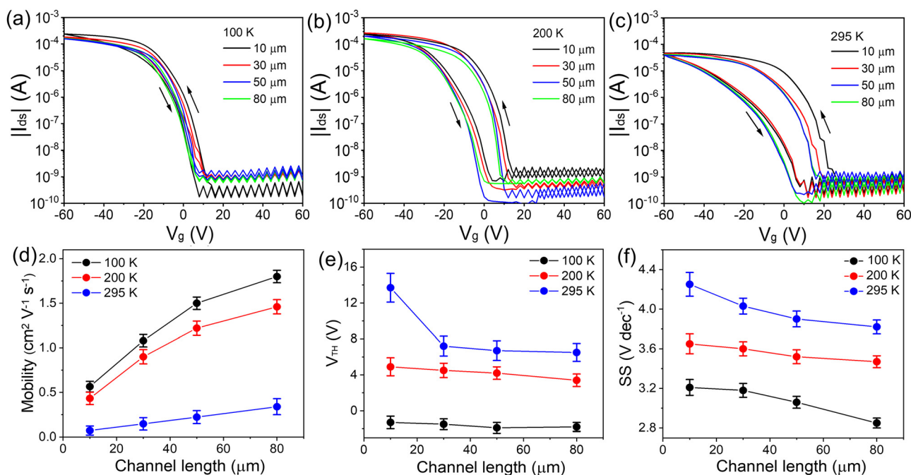
Fig. 6 Transfer characteristics measured at (a) 100 K, (b) 200 K, and (c) 295 K of 120^\circ \text{C} hot-casting (\text{TEA})_2\text{SnI}_4 FETs with different channel lengths L from 10–80 \mu\text{m} and constant W = 1000 \mu\text{m} . (d) Average charge carrier mobility, (e) threshold voltage, and (f) subthreshold swing as a function of channel length measured for (\text{TEA})_2\text{SnI}_4 FETs at 100 K, 200 K and 295 K. The error bars were calculated from 12 devices.
