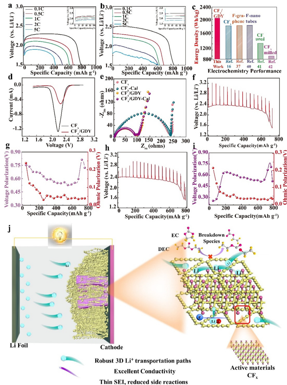
Fig. 3 (a and b) Rate performances of CF x and CF x /GDY hybrids. (c) Comparison of energy densities of CF x /GDY with the reported literature. (d) Cyclic voltammograms and (e) the electrochemistry impedance spectra (EIS). The GITT curves of CF x (f) and CF x /GDY hybrids (h) and the related voltage and ohmic polarization curves derived from the GITT plots of various electrodes (g and i). (j) Schematic illustration of the reaction mechanism for CF x /GDY hybrids.
