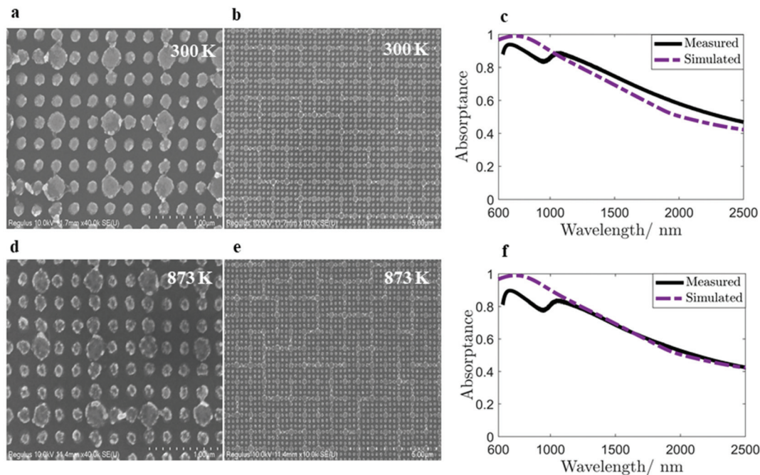
Fig. 3 SEM images of the absorber and the measured absorbance (a) at 300 K with a scale bar of 1 μm and (b) at 300 K with a scale bar of 5 μm. (c) Comparison of the measured and simulated absorbances at 300 K, (d) at 873 K with a scale bar of 1 μm, and (e) at 873 K with a scale bar of 5 μm. (f) Comparison of the measured and simulated absorbances at 873 K.
