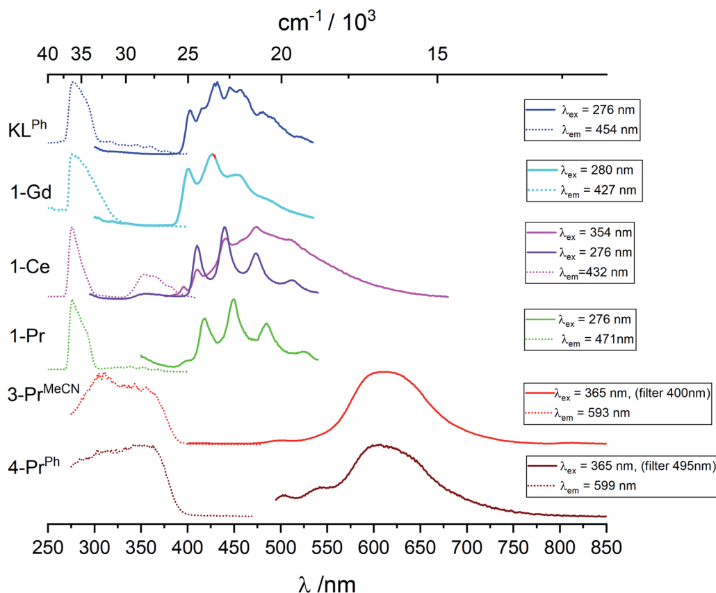
Fig. 5 Excitation and emission spectra of \text{KOSiPh}_3 , 1-Ln (Ln = Gd, Ce, Pr), 3-Pr MecN and 4-Pr Ph in 5 mM toluene solution at 77 K. Spectra are normalized and their intensities cannot be directly compared.
