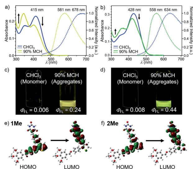
Fig. 2 (a) and (b) UV/Vis absorption (left axis) and fluorescence spectra (right axis, excited at 377 nm for 1 and 392 nm for 2) of (a) 1 and (b) 2 in MCH/CHCl 3 mixture (MCH fraction = 0% and 90%) (c = 100 \mu M). (c) and (d) Photographs of (c) 1 and (d) 2 in CHCl 3 (left) and 90 : 10 MCH/CHCl 3 (v/v) mixture (right) under 365 nm light illumination (c = 100 \mu M). (e) and (f) Molecular orbitals of the S_0 \rightarrow S_1 transition for model compounds (e) 1Me and (f) 2Me (see ESI†) calculated at the TD-CAM-B3LYP/6-31+G(d,p) level of theory. The molecular structures of 1Me and 2Me were optimized by DFT calculation at the CAM-B3LYP/6-31+G(d,p) level of theory. For all calculations, dodecyl groups were replaced with methyl groups.
