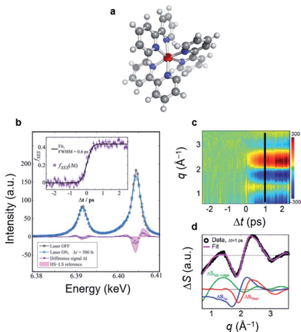
Fig. 12 (a) Chemical structure of [\text{Fe}(\text{bpy})_3]^{2+} . (b) Measured \text{K}\alpha TR-XES spectrum of the ground-state (laser OFF) and photoexcited (laser ON) [\text{Fe}(\text{bpy})_3]^{2+} with the difference spectrum at 500 fs time delay. The static difference spectrum obtained from the spectra of the HS and LS states of a reference sample is shown in the light-purple area. (c) Fs-TRXL data of [\text{Fe}(\text{bpy})_3]^{2+} . (d) The fs-TRXL data at 1 ps together with a corresponding fit. The different components contributing to the fitted curve are shown in the bottom part of (d). Reproduced from ref. 71 with the permission of the American Chemical Society, copyright 2016.
