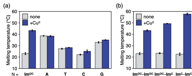
Fig. 5 Melting temperatures of duplexes containing an \text{Im}^{\text{OC}}\text{-N} base pair ( 1 · 2N ; \text{N} = \text{A}, \text{T}, \text{C}, \text{G} ) in the absence and presence of 1 equiv. of \text{Cu}^{\text{II}} . (b) Melting temperatures of duplexes containing an \text{Im}^{\text{OC}}\text{-Im}^{\text{OC}} ( 1 · 2 ), an \text{Im}^{\text{OC}}\text{-Im}^{\text{C}} ( 1 · 8 ), or an \text{Im}^{\text{C}}\text{-Im}^{\text{C}} base pair ( 7 · 8 ) in the absence and presence of 1 equiv. of \text{Cu}^{\text{II}} . [duplex] = 2.0 \mu\text{M} and [\text{Cu}^{\text{II}}]/[\text{duplex}] = 0 or 1 in 10 mM HEPES buffer (pH 7.0) and 100 mM NaCl. N = 3 . The error bars represent the standard errors.
