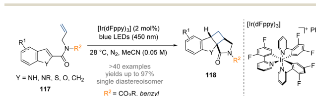
Scheme 34 Dearomative photoredox catalysed intramolecular [2 + 2] cycloaddition of indoles. 40
