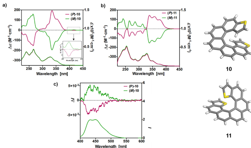
Fig. 3 The experimental UV-vis (bottom) and ECD (top) spectra of the (P) and (M) isomers of 10 and 11 ( CH_2Cl_2 , C \sim 10^{-5} M) are shown in panels (a) and (b), respectively. The inset in (a) shows the magnified ECD of (P) and (M)- 10 in the 400–450 nm region. The fluorescence (bottom) and CPL (top) spectra of (P) and (M)- 10 are shown in panel (c).
