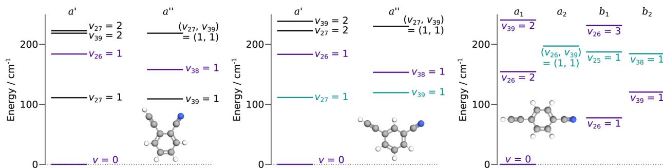
Fig. 2 Lowest energy level diagram of o -, m -, and p -CEB, from left to right, as a function of symmetry. Only states lying below 250 cm -1 are represented. Pure rotational transitions within states represented in purple have been assigned in this study. For the states represented in blue-green, tentative assignments are proposed. Energy of states involving several quanta of excitation are obtained by summing the energies of each associated state with a single quantum of excitation.
