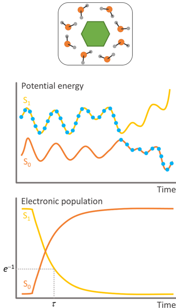
Fig. 1 Schematic features of surface hopping. Top: Molecular system. Middle: Single trajectory representation of the potential energies as a function of time. The dots indicate the populated state at each step. Bottom: Statistics over all independent trajectories allow for estimating each state's electronic population as a function of time and determining the time constant for the internal conversion ( \tau ).
