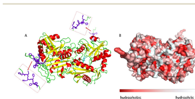
Fig. 2 A: Visualization of the secondary structure of N-terminal His-tagged (R)-selective \omega -transaminase from Arthrobacter sp. (His 6 -ATA-117). In purple the histidine tag and in cyan the PLP cofactor, enzyme diameter: 7.17 nm. B: Surface hydrophobicity: in red the hydrophobic areas and in light-grey the hydrophilic areas. The enzyme structure was predicted using AlphaFold software, figures and the enzyme diameter was obtained using PyMOL software.
