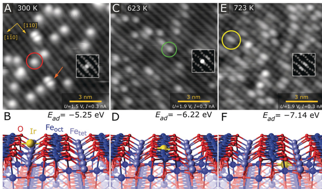
Fig. 5 (A) \text{Ir}_1 atoms evaporated directly onto the \text{Fe}_3\text{O}_4(001) surface at 300 K, which are imaged as bright protrusions between the Fe rows of the support (red circle in STM image). (B) DFT-derived minimum-energy structure of the two-fold-coordinated Ir adatom on \text{Fe}_3\text{O}_4(001) . (C) After annealing at 623 K, Ir atoms appear as bright protrusions within the Fe row in the STM image (green circle). (D) DFT-derived minimum-energy structure of the five-fold-coordinated Ir atom incorporated within the \text{Fe}_3\text{O}_4(001) surface. (E) At 723 K, some of the bright protrusions within the row are replaced by extended bright protrusions in STM (yellow circle). (F) DFT-derived minimum-energy structure of the six-fold-coordinated Ir adatom incorporated in the subsurface layer of \text{Fe}_3\text{O}_4(001) . Reproduced with permission. 24 Copyright © 2019 The Authors. Published by Wiley-VCH Verlag GmbH & Co. KGaA.
