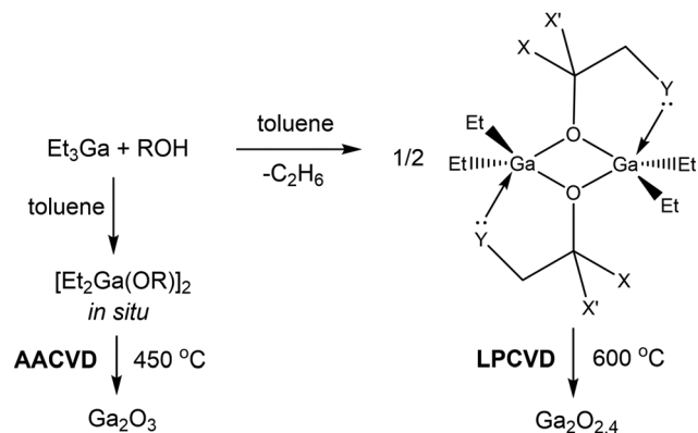
Fig. 18 In situ precursor formation, using AACVD and lower process temperature, versus pre-deposition synthesis, isolation, and purification; R = CH 2 CH 2 NMe 2 , CH(CH 3 )CH 2 NMe 2 , C(CH 3 ) 2 CH 2 OMe, or CH(CH 2 NMe 2 ) 2 , X and/or X' = H, CH 3 , or CH 2 NMe 2 ; Y = NMe 2 or OMe. 230
