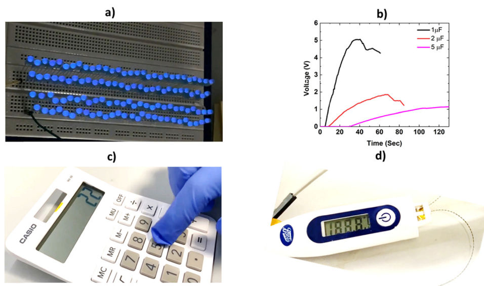
Fig. 6 TENG applications – (a) powering up 115 LEDs, (b) charging capacitors, (c) powering a digital calculator and (d) a thermometer.
