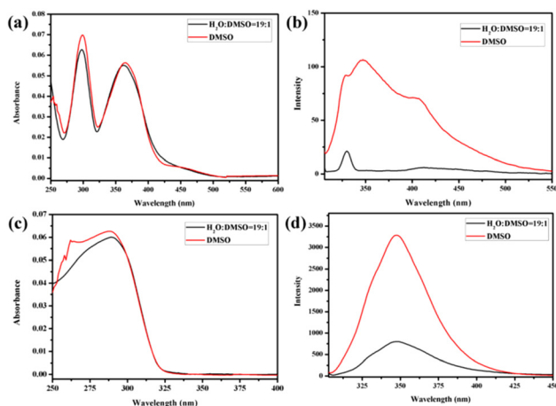
Fig. 1 The absorption spectra of (a) H 1 and (c) H 2 , and emission (excited at 298 nm, Ex bandwidth: 2.5 nm; Em bandwidth: 5 nm) spectra of (b) H 1 and (d) H 2 in DMSO and H 2 O/DMSO (v/v = 19:1) solutions ( 3.03 \times 10^{-6} mol L -1 ).
