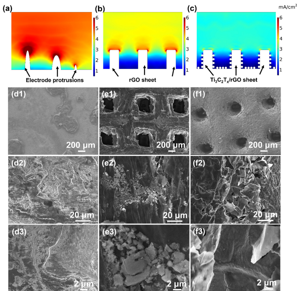
Fig. 4 Surface current density distribution simulated by COMSOL Multiphysics on (a) Cu, (b) 3D-printed rGO and (c) 3D-printed 50% Ti_3C_2T_x /rGO electrodes. SEM images of (d) Cu, (e) 3D-printed rGO and (f) 3D-printed 50% Ti_3C_2T_x /rGO electrodes after 100 cycles at 2 \text{ mA cm}^{-2} with 2 \text{ mA h cm}^{-2} .
