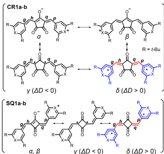
Fig. 6 Resonance structures of CR1a–b and SQ1a–b . Red-highlighted parts indicate methine parts (bonds g , h , p , and q ) with bond length alternation. Blue-highlighted parts are chalcogenopyrylium rings in which unpaired electrons are delocalized. The difference between bond lengths at methine parts \Delta D is obtained as follows; \Delta D = (\text{averaged length of } g, p) - (\text{averaged length of } h, q) .
