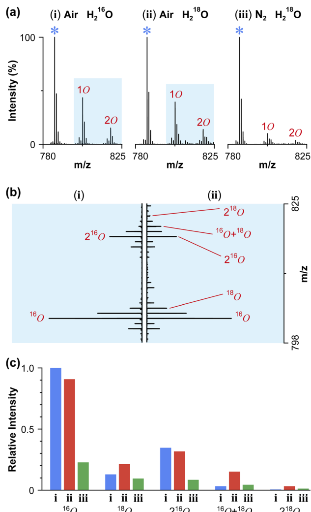
Fig. 8 Measurement using the oxygen isotope. (a) Mass spectra obtained under oxidized conditions for 5 \mu\text{M} L-phosphatidylcholine (PC 18:1/18:1) in 500 mM HCl prepared using normal water (i) and water- ^{18}\text{O} (ii & iii). The operating gases are air (i & ii) and high-purity nitrogen (iii). Asterisk denotes the peak without oxidation. (b) Enlarged view of (a) (i) and (a) (ii). (c) Intensity comparison for different oxidation species.
