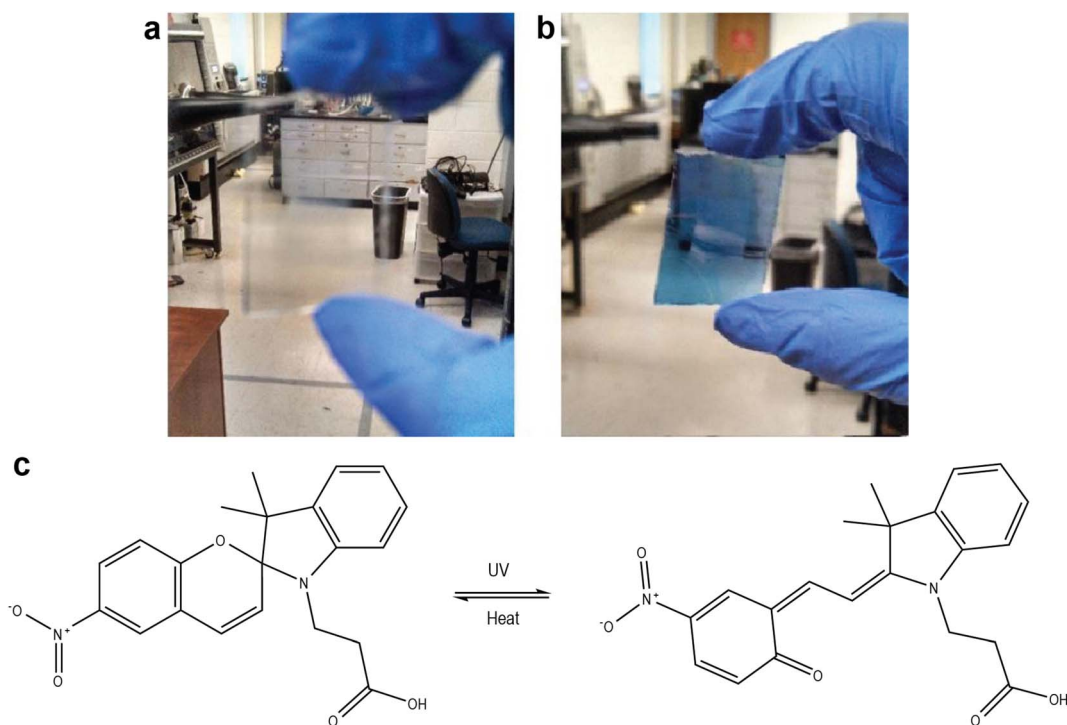
Fig. 4 Color change of a spiropyran dye on a TiO 2 film (a) before and (b) after exposure to sunlight. DSCs fabricated using this dye showed power conversion efficiencies of 0.007% (clear) and 0.028% (colored). (c) Chemical structures of the dyes shown above. Figure adapted with permission from ref. 31. Copyright 2015 by Johnson et al., licensee AIMS Press.
