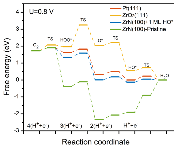
Fig. 2 Calculated free energy diagrams of the ORR at pristine ZrN(100) and ZrN(100) covered by 1 ML HO*, Pt(111), 40 and ZrO 2 (111). 19 The energy barriers of the elementary steps were estimated based on the method by Dickens et al. 41 The potential was set to 0.8 V vs. RHE.
