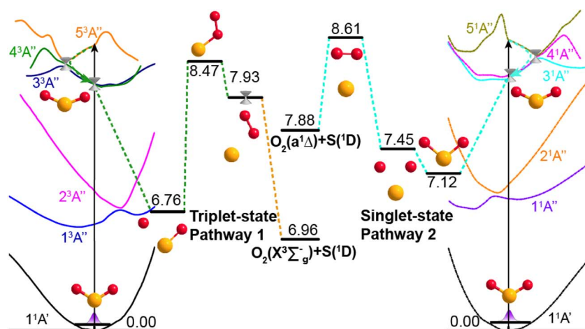
Fig. 4 Dissociation pathways of \text{SO}_2 leading to \text{O}_2(\text{X}^3\Sigma_g^-) + \text{S}^1\text{D} products via the triplet state manifold (left) and to \text{O}_2(\text{a}^1\Delta_g) + \text{S}^1\text{D} products via the singlet state manifold. The schematics of the simplified PECs for the ground and the first five excited states of ^3\text{A}'' symmetry (left) and the first five states of ^1\text{A}'' symmetry (right) support different paths leading to \text{S} + \text{O}_2 product formation. Dashed arrows indicate possible non-adiabatic pathways and the geometries and energies (in eV) of key intermediate structures along the dissociation pathways are also indicated. The horizontal axis represents the reaction coordinate, and the vertical axis is the potential energy (in eV).
