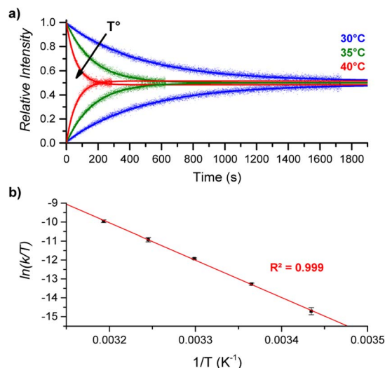
Fig. 4 (a) Relative time evolution of [CoC(Py IN )] + (top lines) and [CoC(Py OUT )] (bottom lines) in DRL experiments carried out in CHCl 3 at 30 °C (blue), 35 °C (green), and 40 °C (red). Dots are experimental data points, and lines correspond to fittings of experimental data by eqn (S1) and (S2).† (b) Eyring plot built from DRL experiments carried out at different temperatures. Dots correspond to the average of ln(k/T) values from triplicate measurements, with error bars corresponding to the standard deviation.
