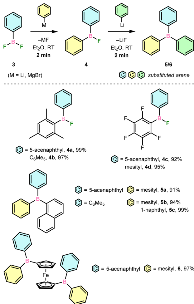
Scheme 3 Isolated yields of transmetallations with aryldifluoroboranes ( 3 ) to form di- ( 4 ) and triarylboranes ( 5–7 ). [a] Reaction was run in pentane at -35\text{ }^{\circ}\text{C} .
