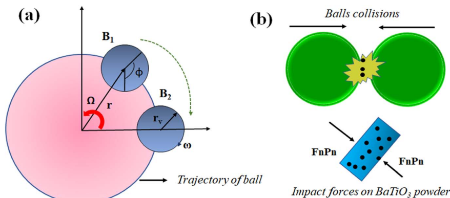
Fig. 10 (a) Trajectory of balls in planetary motion, (b) mechanics of balls for generating piezocatalysis in BaTiO 3 powder.
