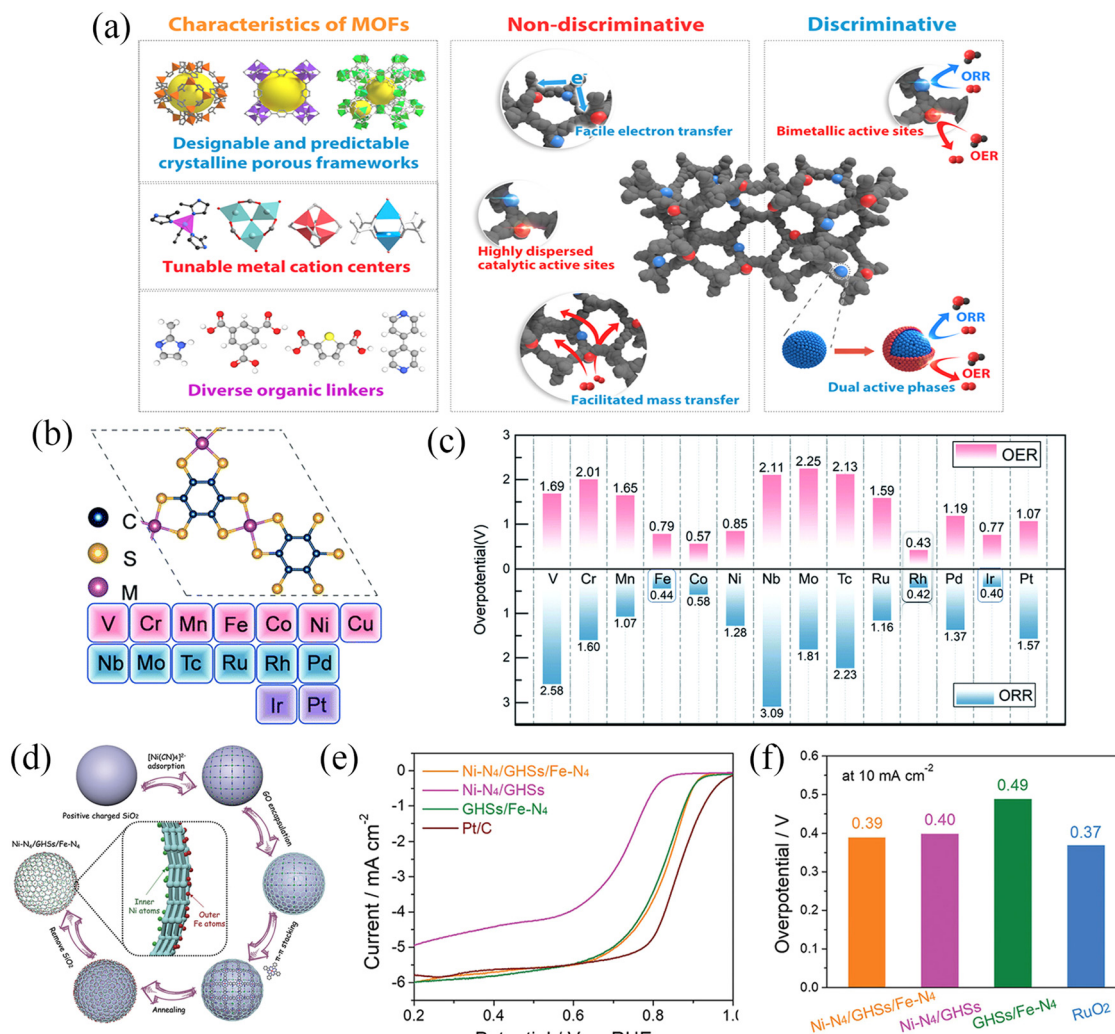
Fig. 15 (a) Schematic illustration of the outstanding features of MOFs and their derivatives in OER and ORR application. (Reproduced from ref. 148 with permission from Elsevier). (b) Schematic illustration of M_3(C_6S_6)_2 with different transition metals. (c) OER and ORR overpotentials of M_3(C_6S_6)_2 . (Reproduced from ref. 150 with permission from the Royal Society of Chemistry). (d) Synthesis procedure for the Ni-N 4 /GHSs/Fe-N 4 catalyst. (e) The ORR results and (f) the OER results of different catalysts. (Reproduced from ref. 151 with permission from Wiley).
