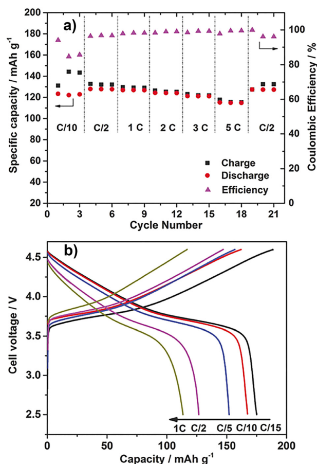
Fig. 10 Electrochemical measurements of 40 wt% \text{Li}_{0.110.9}\text{b} /PVDF composites. (a) Specific capacities and coulombic efficiencies of \text{Li}/\text{LiFePO}_4 cells at different current rates, ranging from C/10 to 5C, 50 ^{\circ}\text{C} . (b) Charge-discharge curves of the \text{Li}/\text{LiCo}_{1/3}\text{Ni}_{1/3}\text{Mn}_{1/3}\text{O}_2 cell using 40 wt% \text{Li}_{0.110.9}\text{b} /PVDF composites (cut-off voltage 2.5–4.6 V), 50 ^{\circ}\text{C} . (Figure partly modified from the original one.) Reprinted from ref. 94 with permission.
