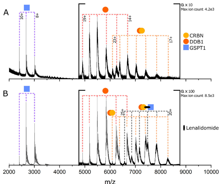
Fig. 2 (A) GSPT1 + CRBN:DDB1 (B) GSPT1 + CRBN:DDB1 + lenalidomide. Protein concentrations are 5 \mu M and lenalidomide is 100 \mu M when present. Measured masses of the labelled species are as follows: GSPT1 24 058 Da. DDB1 93 247 Da. CRBN:DDB1 139 775 Da. Ternary complex 164 090 Da. Masses given to the nearest 1 Da, and further details are given in Table S2. †
