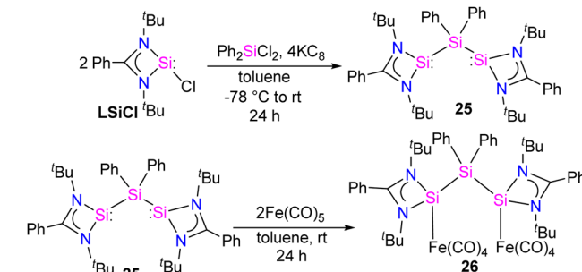
Scheme 8 Synthesis of 25 and 26 .
