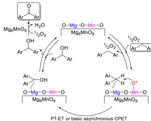
Fig. 11 Proposed reaction mechanism for the catalytic oxidation over Mg_6MnO_8 -MA with O_2 . O^* : schematic representation of surface oxygen species ( O_2^- , O_2^{2-} , O^{2-} , OH^- etc.). (Reproduced from ref. 46 with permission from The American Chemical Society).
