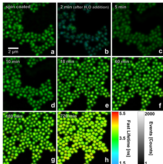
Fig. 1 Confocal FLIM images of ATTO 655 labelled P(NIPAM- co -APMH) microgels measured (a) after spin-coating, and (b)–(h) at different drying times (indicated in the images) at open atmospheric pressure after the addition of a small amount of \text{H}_2\text{O} at time zero, respectively. FLIM images of additional times are presented in Fig. S1 in the ESI.† The field of view changes between (d) and (e) since two different measurements (one concentrating on a high sampling of the short times and the other addressing the long time behaviour) were combined.
