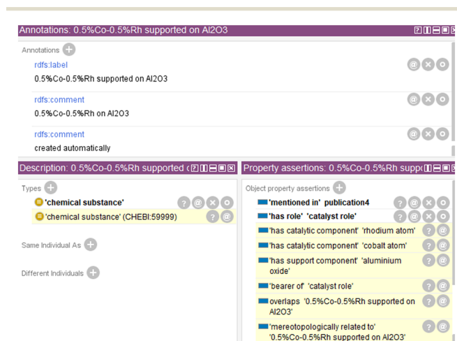
Fig. 6 Excerpt from Protégé with inferred relations after reasoning for the individual “0.5% Co–0.5% Rh supported on \text{Al}_2\text{O}_3 ”. Knowledge inferred by the reasoner is highlighted in yellow, showing increased semantic expressiveness of the individual.
