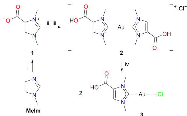
Scheme 2 Preparation of di- and monocarbene gold(II) complexes from norzooanemonin ( 1 ); reagents and reaction conditions: (i) 1 equiv. dimethyl carbonate, bomb flask, 8 h, 140 °C; (ii) 1 equiv. K_2CO_3 , 0.5 equiv. (Me_2S)_2AuCl , MeOH, 12 h, rt; (iii) HCl (2 N), pH = 1–2, H_2O , rt; (iv) 1 equiv. (Me_2S)_2AuCl , MeOH, 4 h, rt.
