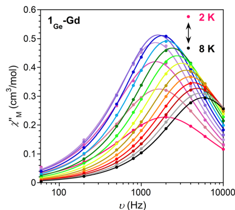
Fig. 2 Frequency dependence of the out-of-phase component of the ac susceptibility at H_{\text{dc}} = 2500\text{ Oe} for 1 Ge -Gd . The experimental data are denoted by circles; solid lines represent the best fit to the data.
