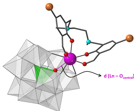
Fig. 1 Molecular structure of hybrid [\text{Ln}(\text{H}_2\text{L})(\alpha\text{-GeW}_{11}\text{O}_{39})]^{5-} anions in 1 Ge -Ln . The \text{Ln}\cdots\text{O}_{\text{central}} bond is represented as a purple line and discussed in the text. Colour code: \text{WO}_6 , grey; \text{GeO}_4 , green; Ln, purple; C, black; O, red; N, blue; Br, orange. H atoms have been omitted for clarity.
