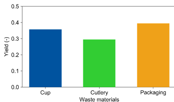
Fig. 4 Yield of lactic acid determined with HPLC for the depolymerisation of real waste materials. Conditions: Pt cathode, Pt anode, 40 \text{ mA cm}^{-2} , 150^\circ \text{C} , dioxane/water (vol. 9 : 1), 0.25 \text{ M LiClO}_4 , 60^\circ \text{C} , 5 \text{ mg mL}^{-1} PLA.
