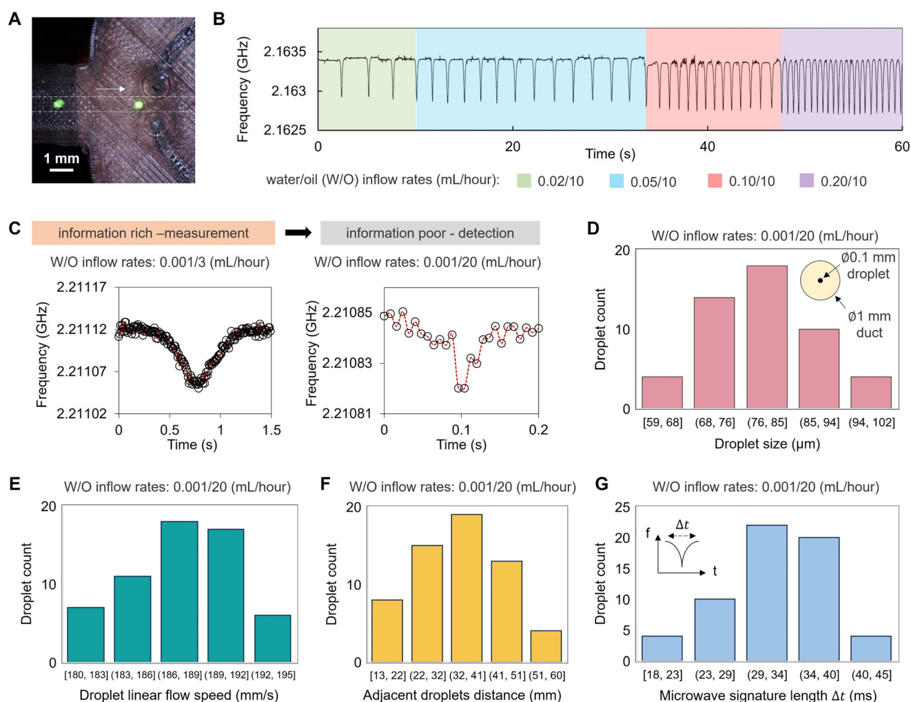
Fig. 3 Performance of the 3D-printed MMD on droplet sensing. A , Neighbouring droplets flowing through the split ring resonator. B , Microwave sensing readout of water droplets flowing in the continuous oil phase at different inflow rates. C , Acquired data points of individual droplets at different inflow rates. The quantity of data points determines either volumetric measurement (information rich) or detection (information poor) of the water droplet in the oil flow using the microwave sensing. D , The size of the smallest water droplets, which can be formed and detected in our 3D-printed MMD experiment setup, is around 60 μm flowing in a 1 mm wide fluidic duct. The linear flow velocity of these droplets is approximately 190 mm s -1 ( E ), and the distance between adjacent droplets is approximately 35 mm ( F ), measured with a high-speed camera. It took approximately 35 ms for the droplet to flow across the microwave sensing region ( G ).
