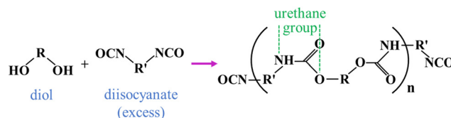
Fig. 1 Reaction scheme of preparing PU.
