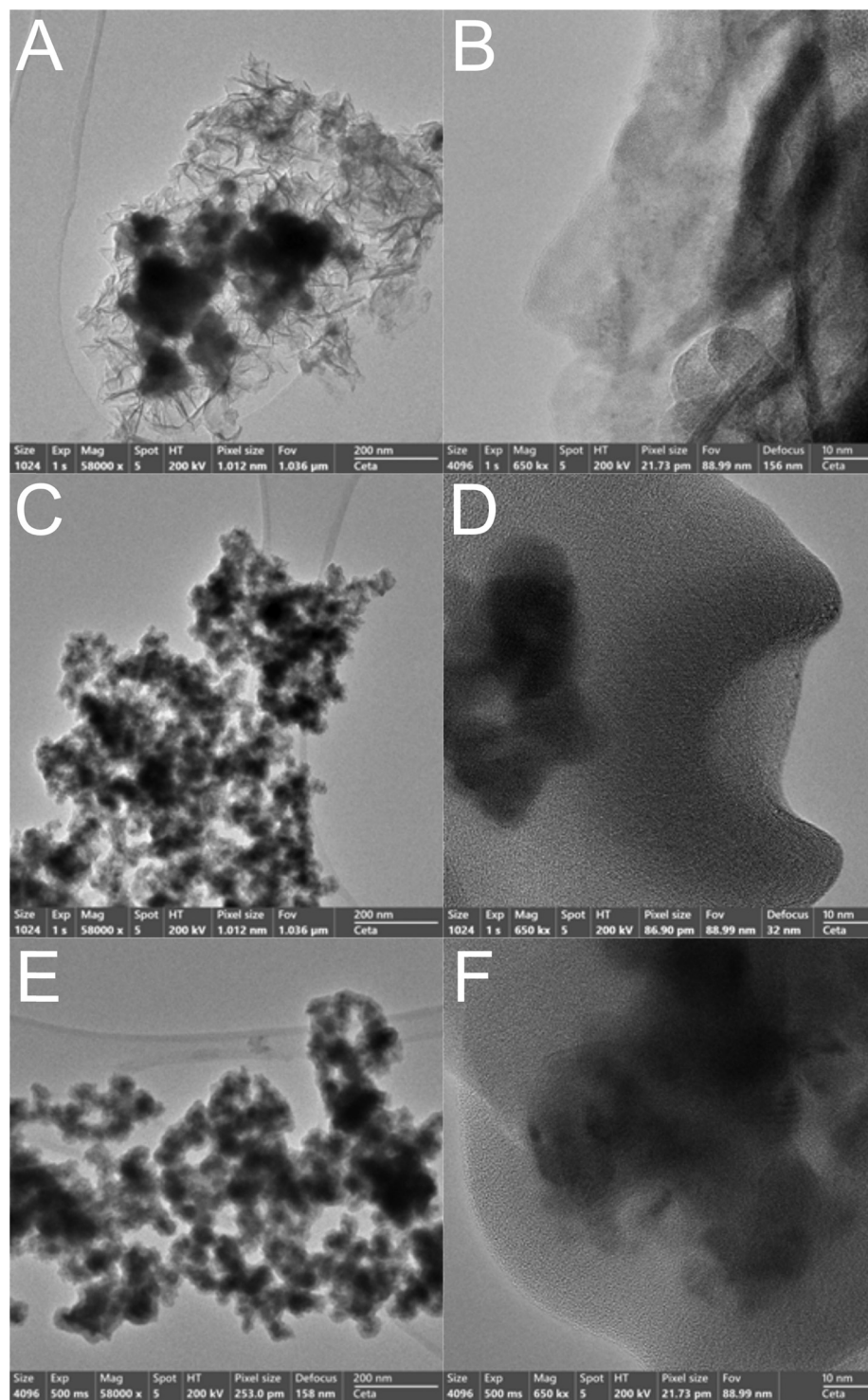
Fig. 1 HR-TEM images at low (left column) and high (right column) magnification (58 Kx and 650 Kx) of NiGra NG1-2-3 samples with increasing load of graphene oxide: (A) and (B) 0.2% GO, (C) and (D) 1% GO, (E) and (F) 5% GO. Scale bar of 200 nm for the low magnification (left column) and 10 nm for the high magnification (right column).
