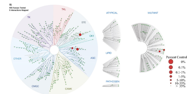
Fig. 4 Kinome tree with 5l kinase selectivity data (data are generated using Discoverex Treespot). A large red circle indicates higher-affinity binding of numerous kinases.
