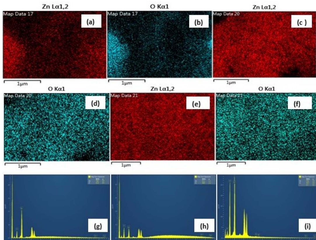
Fig. 6 (a–f) The similar EDX mapping analysis of Zn and O (high purity) in the three samples and (g–i) weight% of Zn, 47.95%; O, 52.05% in nitrate (g), Zn, 39.63%; O, 60.33% in sulphate (h) and Zn, 39.58%; O, 60.42% in acetate (i) (inset, bottom).
